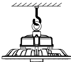
Hanging ring installation
