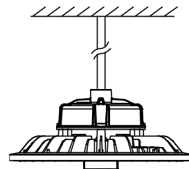
Hanging rod installation
